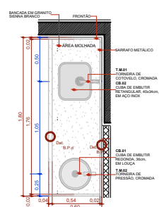
BPC.180e Escala 1:20
