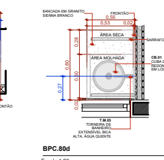
BPC.80d Escala 1:20
