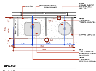
BPC.160 Escala 1:20
