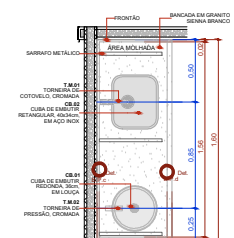
BPC.160d Escala 1:20
