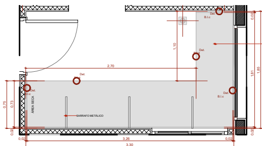
BPC.330de Escala 1:20
