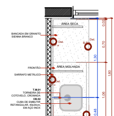
BPC.180d Escala 1:20
